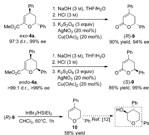
Scheme 4. Transformation of 4a.
