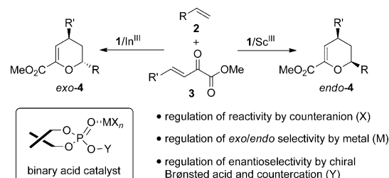
Scheme 1. Diastereoselective and enantioselective [4+2] cycloaddition.
