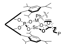
Figure 2. Proposed endo transition state for catalysis with Sc(BArF) 3 /1f.
